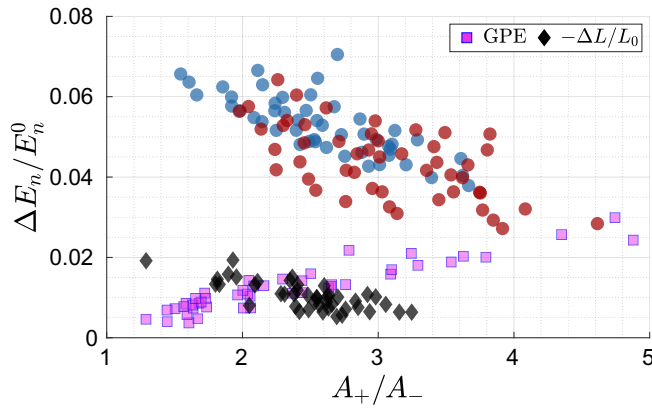
Fig. 4. Normalized energy jumps \Delta E_n/E_n^0 for Hopf link reconnections. The solid black diamonds are the normalized change in line length \Delta L/L_0 in the T = 0 K case. Blue and red circle correspond to T = 1.9 K and T = 2.1 K respectively. The purple squares are from GPE simulations of Villois et al. (11).
