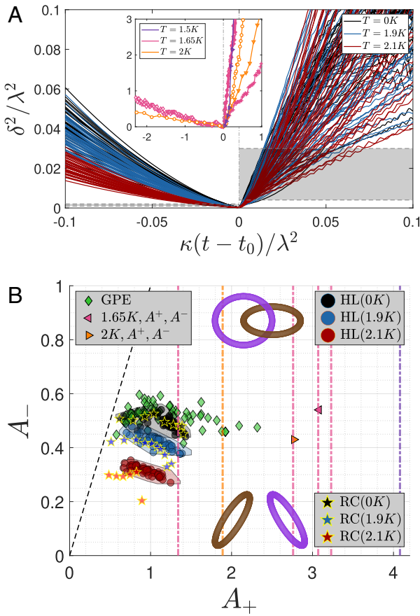
Fig. 2. (A) Time evolution of the (dimensionless) minimum distance squared \delta^2 plotted vs. (dimensionless) \kappa(t - t_0) for the Hopf link reconnections at T = 0K, 1.9K , and 2.1K (black, blue, and red, respectively). The gray shaded areas are the regions used to estimate the prefactors A^\pm . Inset: Experimental superfluid helium data. (B) Comparison of all prefactors: Hopf links (HL, circles), ring collisions (RC, stars with yellow outline), GPE-data from Vilhois et. al. (11) (green diamonds) and experimental results from this study (triangles and vertical dot-dashed lines). The shaded areas associated with each color represent the convex hull of errors for each temperature and the black dashed line represents the theoretical bound for A^+/A^- . Schematic rendering of initial conditions are included.
